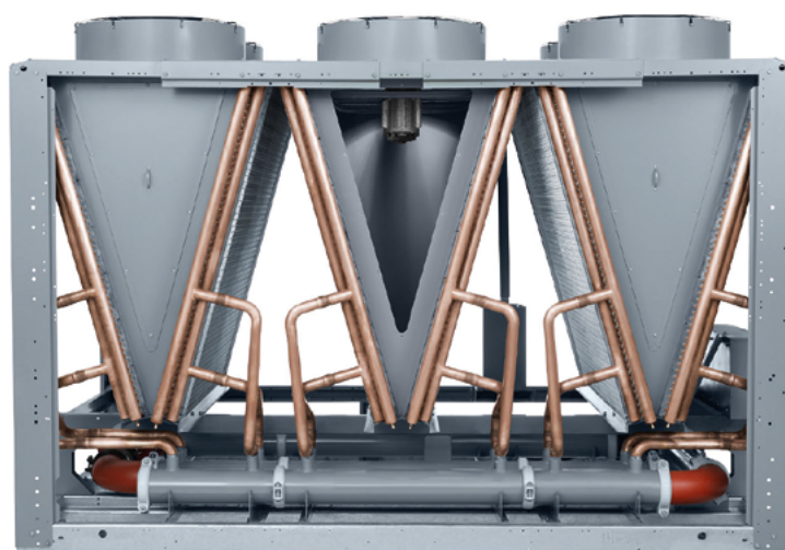
Módulo Free-Cooling
