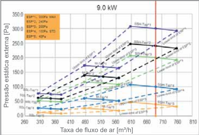
Figura 8.6: MIH90FASHN18
