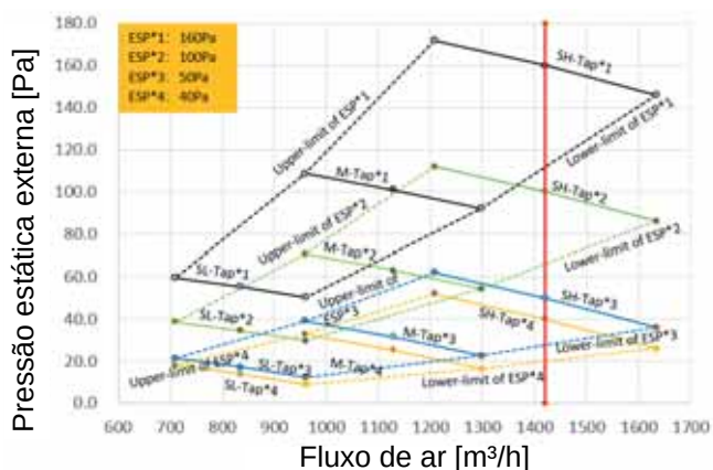
Figura 9.21: MIH90T2HN18
