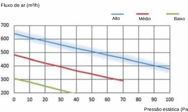
Figura 8.12: HRV-D500(C)
