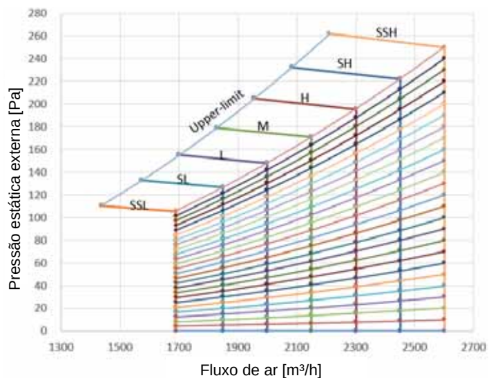
Figura 9.6: MIH160T1HN18
