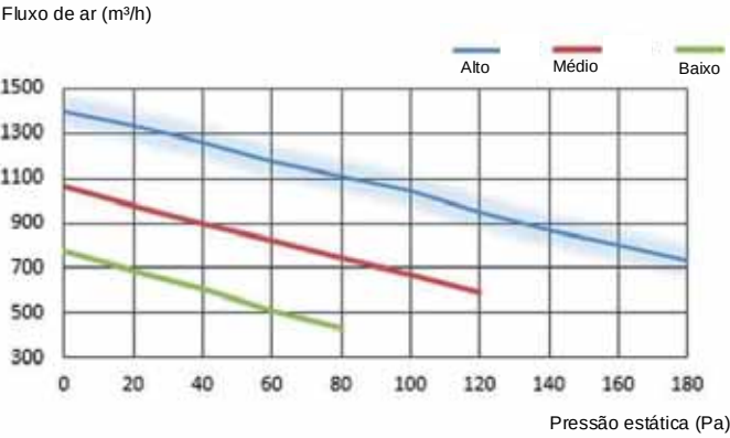
Figura 8.16: HRV-D2000(C)
