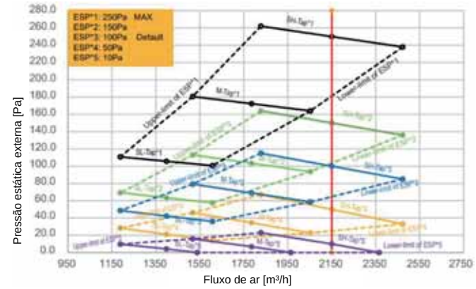
Figura 9.10: MIH125T1HN18
