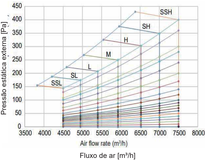
Figura 9.9: MIH400(450)T1HN18
