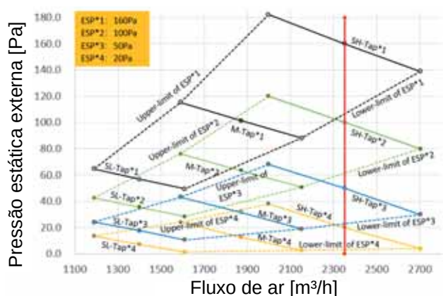
Figura 9.24: MIH160T2HN18
