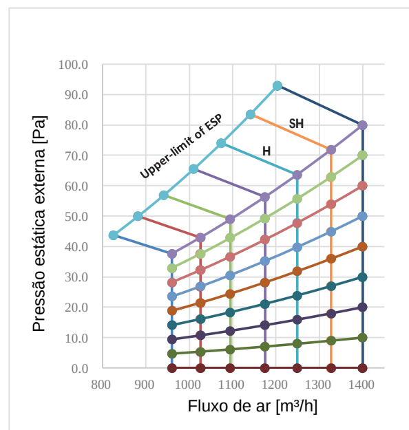
Figura 9.8: MIH80T3HN18
