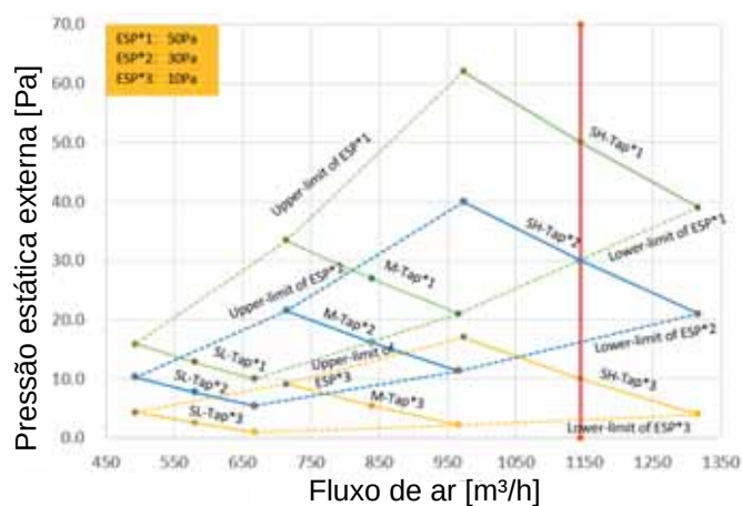
Figura 9.17: MIH71T3HN18
