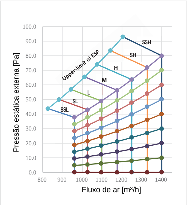
Figura 9.9: MIH90T3HN18
