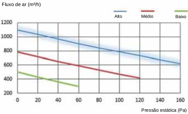
Figura 8.15: HRV-D1500(C)
