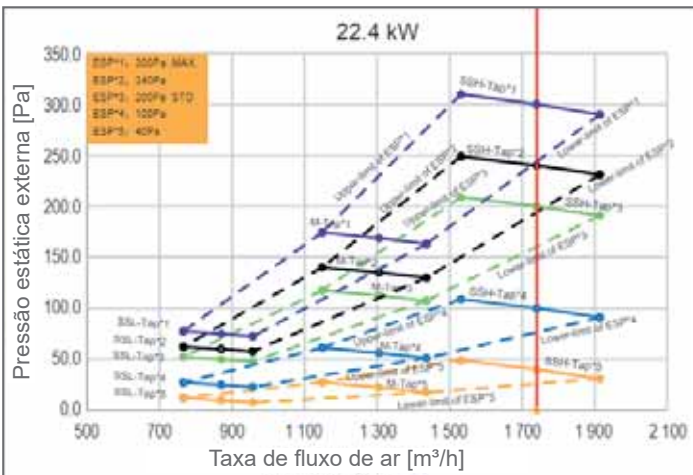
Figura 8.9: MIH224FASHN18
