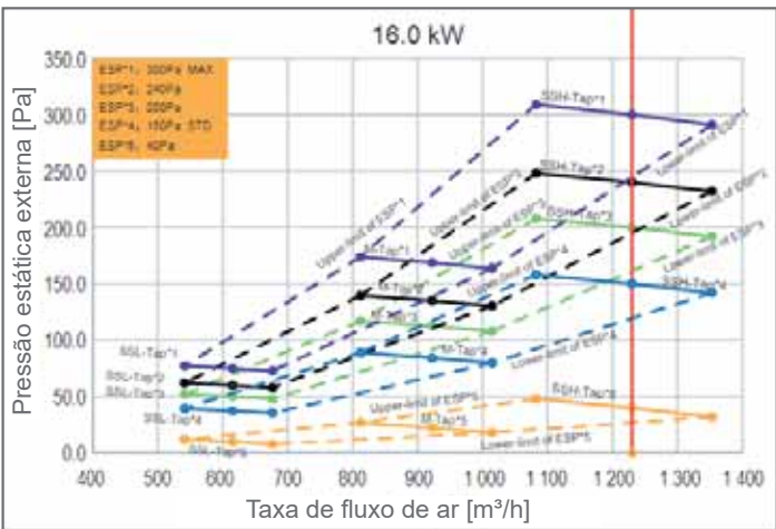
Figura 8.8: MIH160FASHN18
