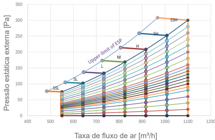
Figura 8.2: MIH140FASHN18
