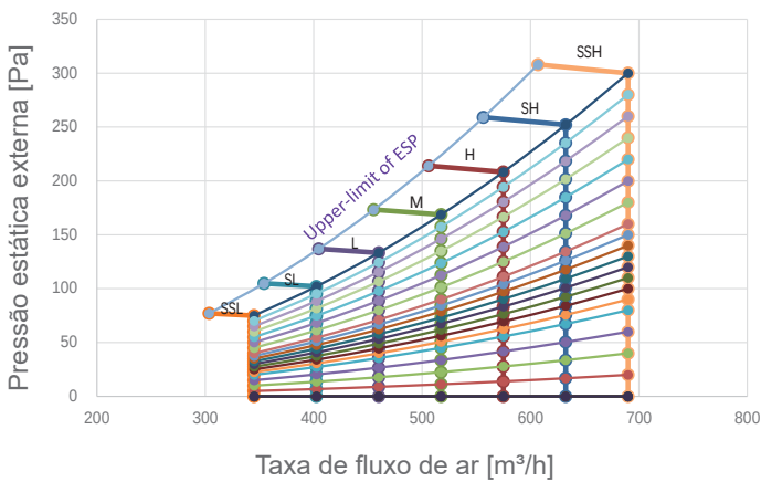
Figura 8.1: MIH90FASHN18
