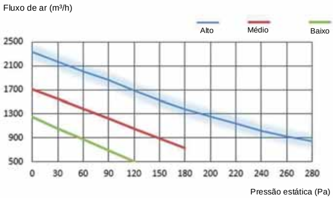
Figura 8.15: HRV-D1500(C)
