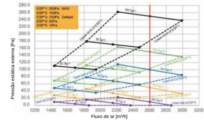
Figura 9.12: MIH160T1HN18
