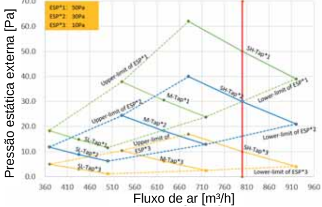
Figura 9.15: MIH45T3HN18
