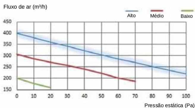
Figura 8.3: HRV-D400(C)
