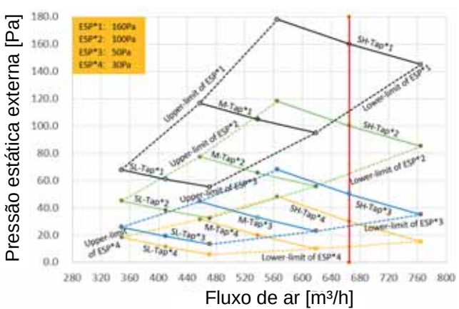
Figura 9.17: MIH45T2HN18
