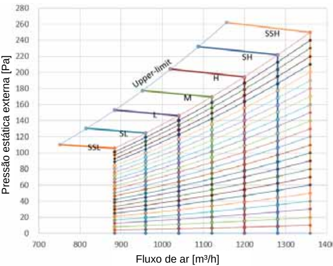
Figura 9.1: MIH56(71,80)T1HN18
