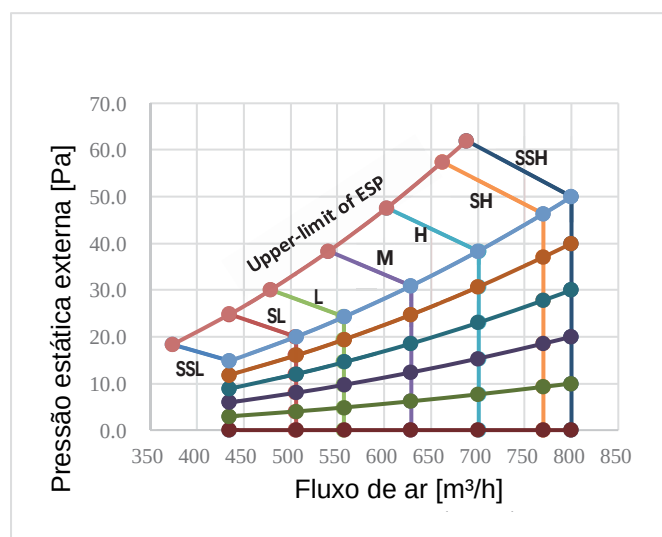
Figura 9.5: MIH45T3HN18
