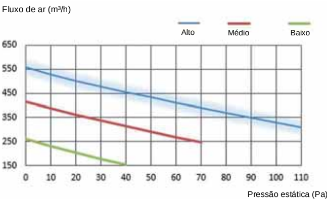
Figura 8.11: HRV-D400(C)
