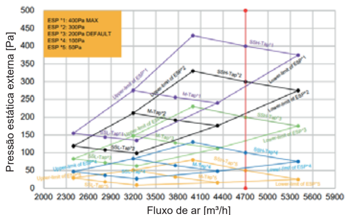
Figura 9.19: MIH400(450)T1HN18
