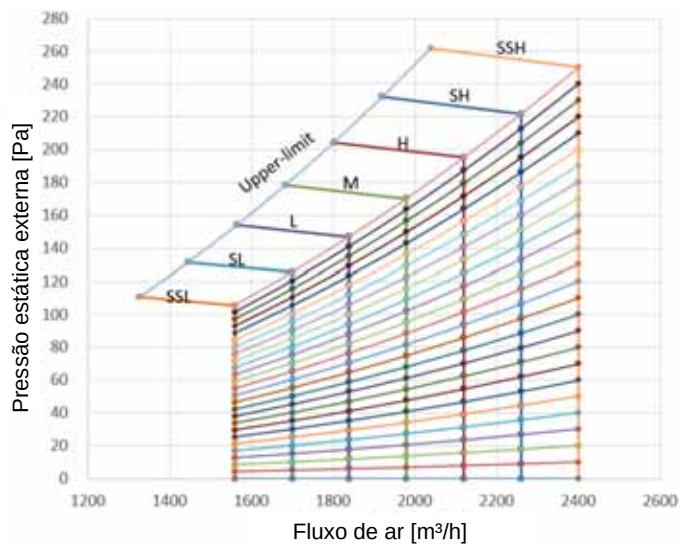
Figura 9.5: MIH140T1HN18
