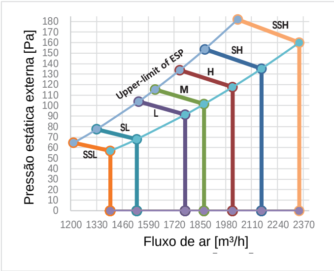
Figura 9.12: MIH160T2HN18
