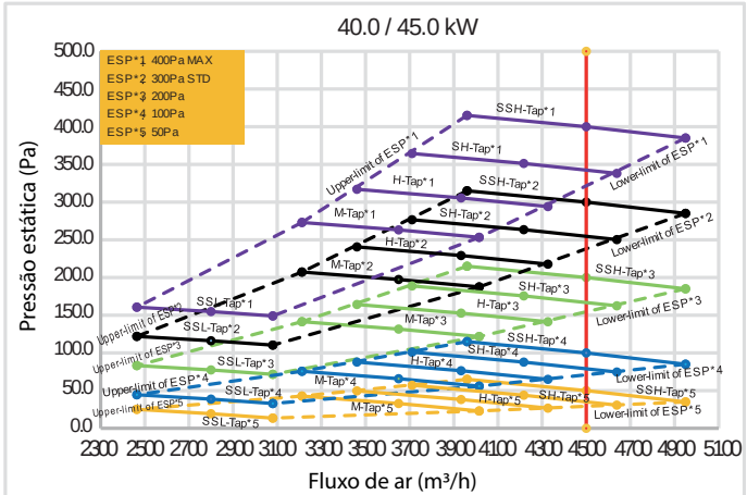
Figura 6.5: Performance do ventilador MIH400(450)FAHN18
