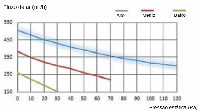
Figura 8.4: HRV-D500(C)
