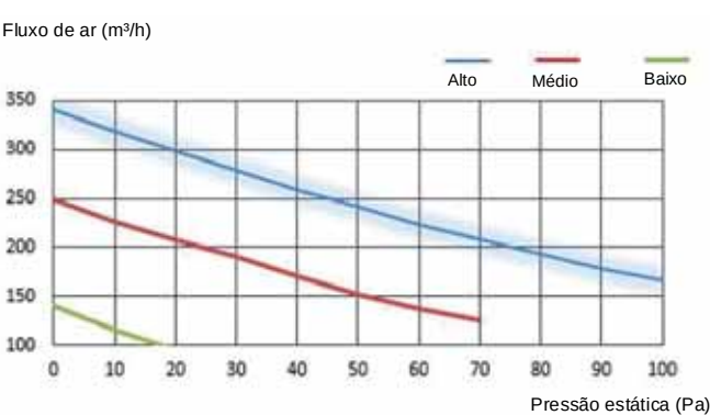
Figura 8.11: HRV-D400(C)
