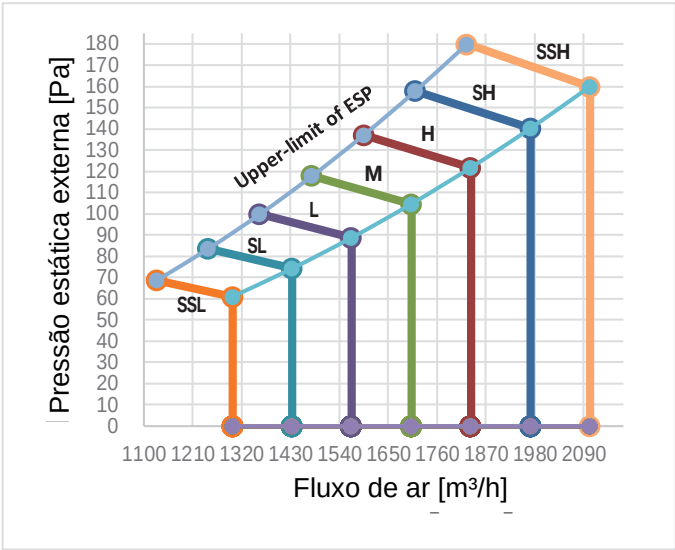
Figura 9.11: MIH140T2HN18
