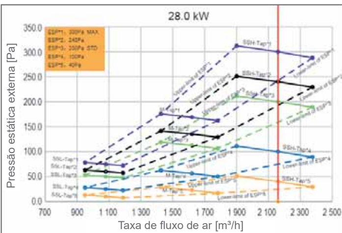
Figura 8.10: MIH280FASHN18
