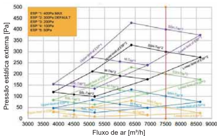
Figura 9.19: MIH400(450)T1HN18
