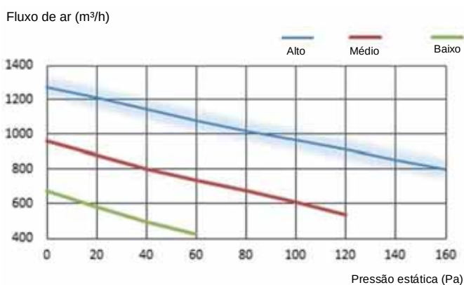
Figura 8.5: HRV-D800(C)
