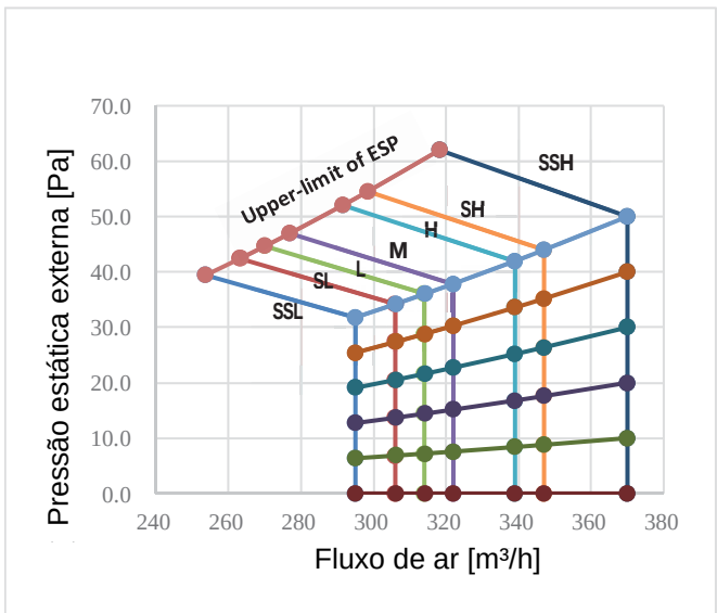
Figura 9.2: MIH22T3HN18
