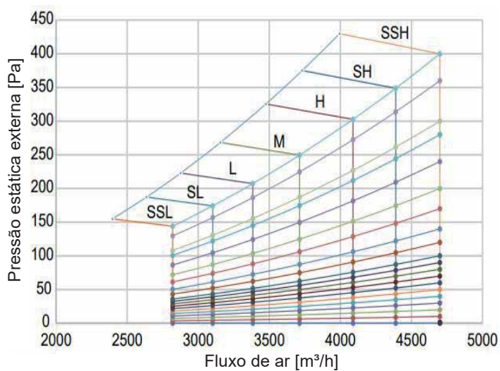
Figura 9.5: MIH335T1HN18
