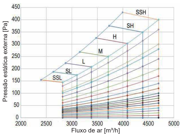
Figura 9.7: MIH200(224,252,280)T1HN18
