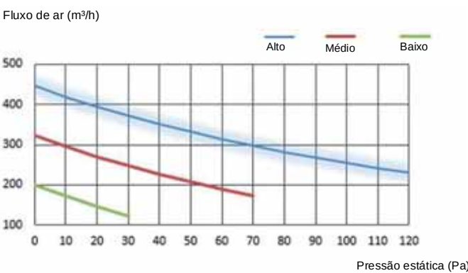
Figura 8.12: HRV-D500(C)
