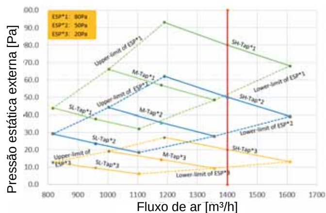
Figura 9.18: MIH80T3HN18
