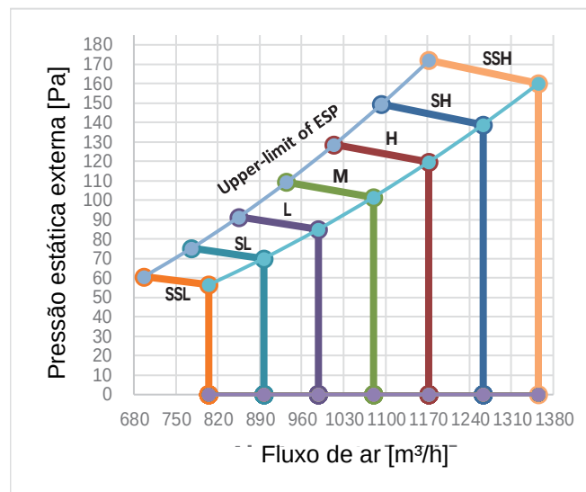
Figura 9.8: MIH80T2HN18
