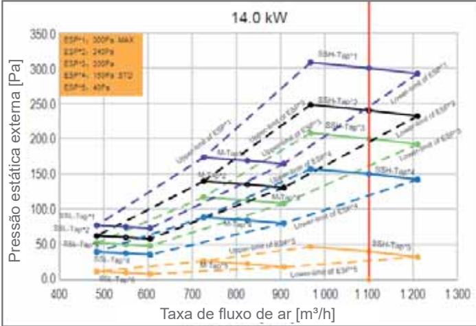
Figura 8.7: MIH140FASHN18
