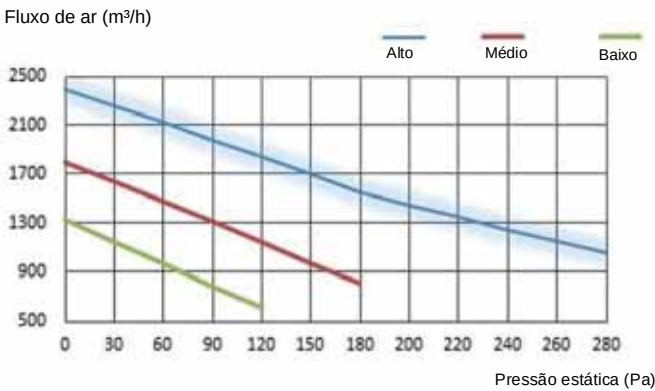
Figura 8.7: HRV-D1500(C)
