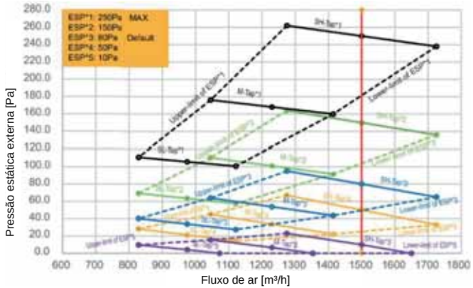
Figura 9.8: MIH90T1HN18
