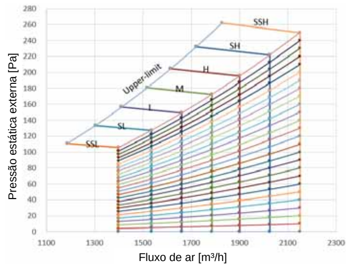
Figura 9.4: MIH125T1HN18
