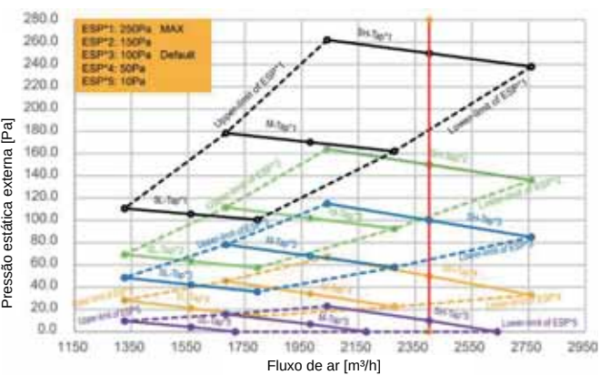
Figura 9.11: MIH140T1HN18
