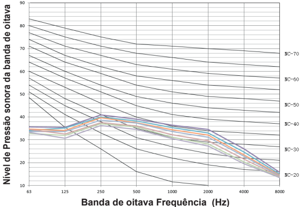
Figura 9.21: MI2-71F5DHN1(A)
