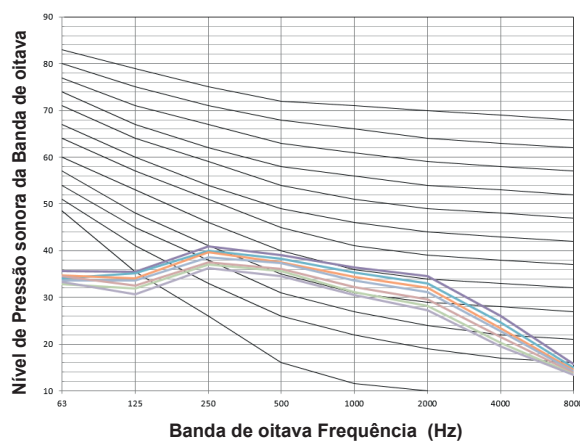
Figura 9.15: MI2-80F4DHN1(A)
