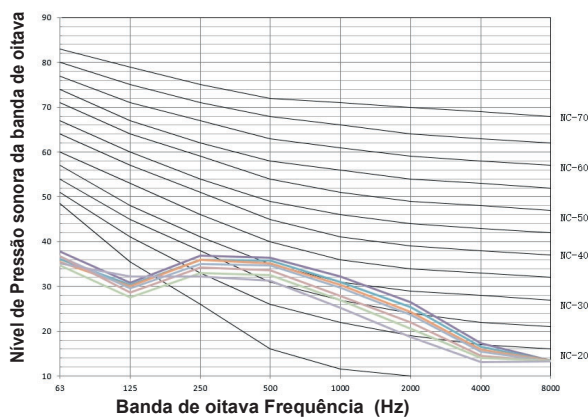
Figura 9.8: MI2-80F3DHN1(A)
