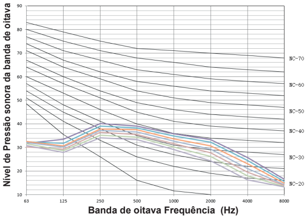
Figura 9.21: MI2-71F5DHN1(A)
