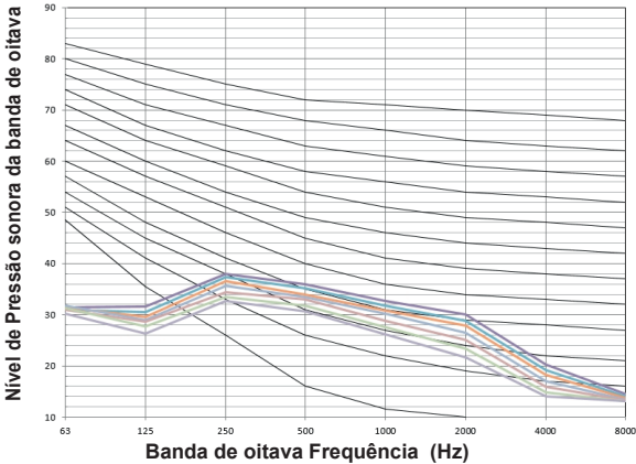
Figura 9.20: MI2-56F5DHN1(A)
