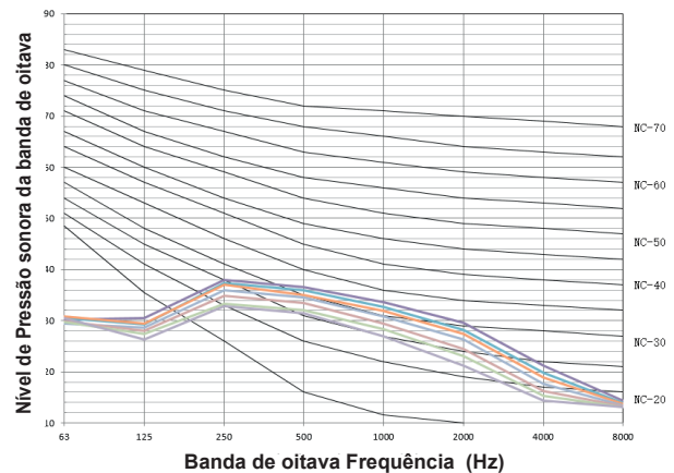
Figura 9.6: MI2-56F3DHN1(A)
