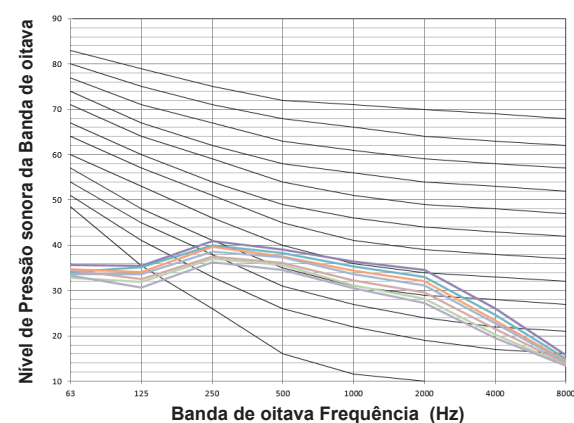
Figura 9.14: MI2-71F4DHN1(A)
