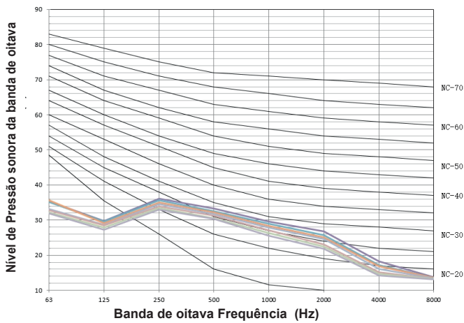
Figura 9.19: MI2-45F5DHN1(A)
