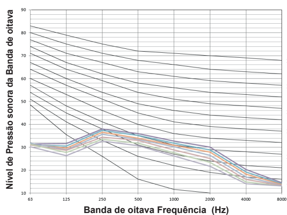
Figura 9.13: MI2-56F4DHN1(A)
