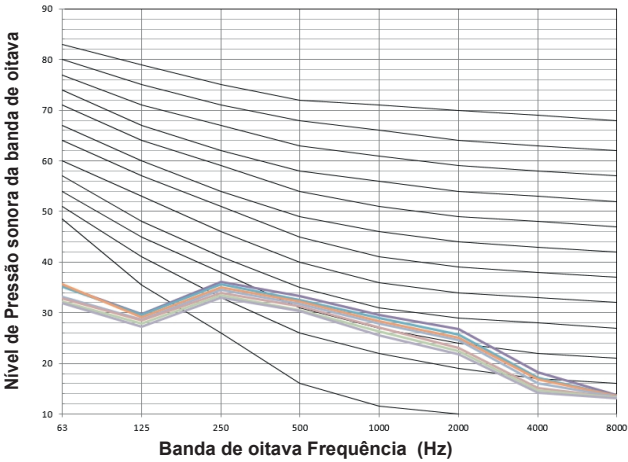
Figura 9.18: MI2-36F5DHN1(A)
