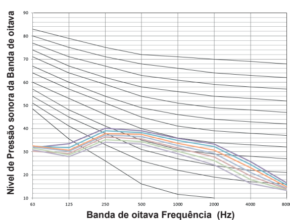
Figura 9.14: MI2-71F4DHN1(A)
