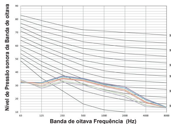
Figura 9.15: MI2-80F4DHN1(A)
