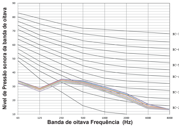
Figura 9.5: MI2-45F3DHN1(A)
