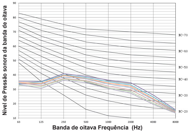
Figura 9.22: MI2-80F5DHN1(A)
