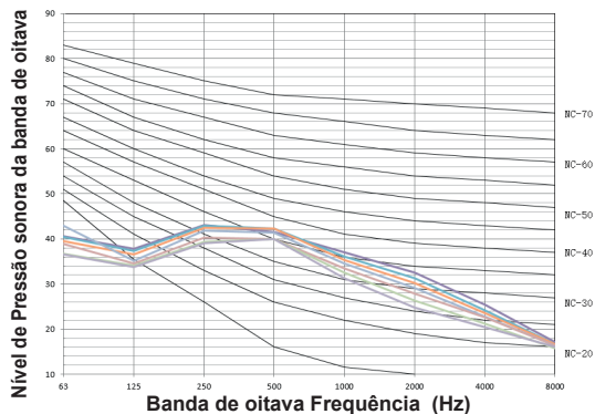
Figura 9.8: MI2-80F3DHN1(A)
