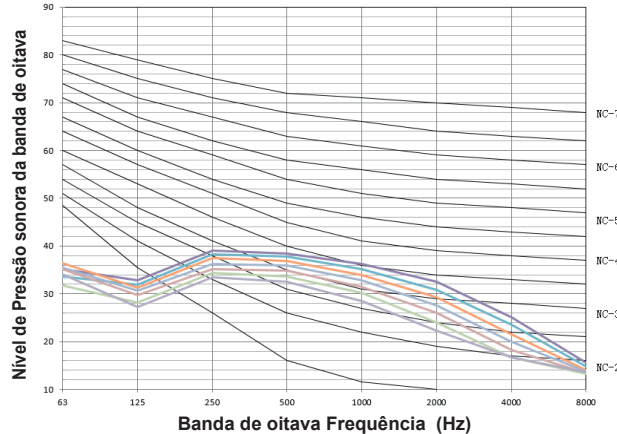
Figura 9.7: MI2-71F3DHN1(A)
