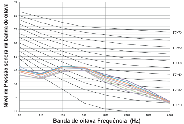
Figura 9.7: MI2-71F3DHN1(A)
