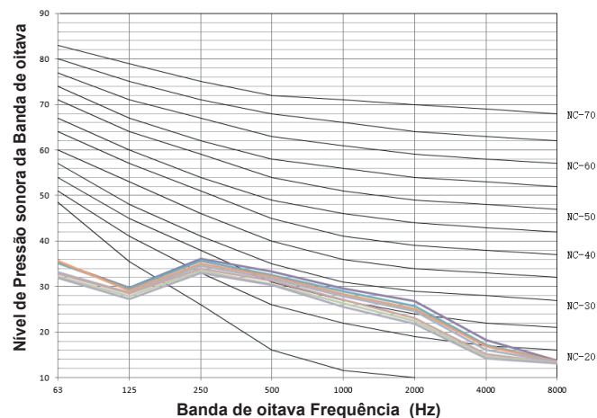
Figura 9.11: MI2-36F4DHN1(A)
