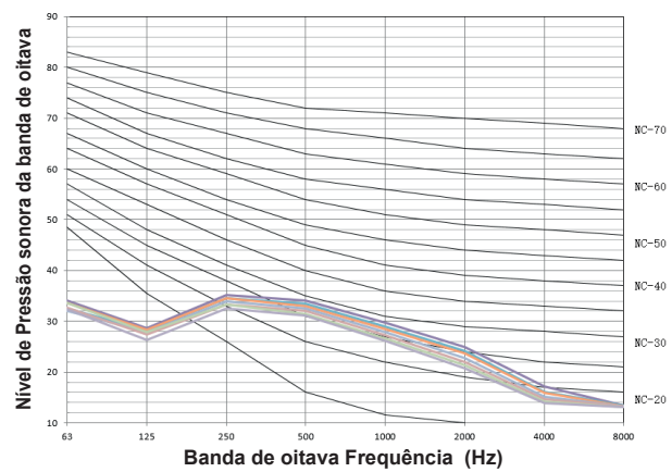
Figura 9.4: MI2-36F3DHN1(A)
