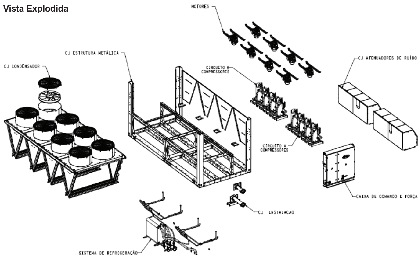
FIG. 1 - Vista explodida 30RSB
